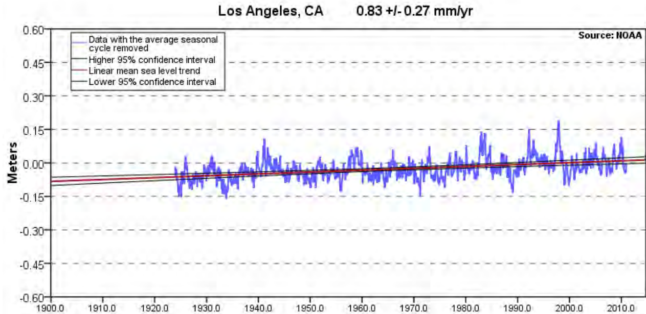
Figure 11.14. Mean sea level trend by decade for Los Angeles, California ( 0.83 \text{ mm/yr} \pm 0.27 ; reproduced NOAA, Sea Levels Online).
