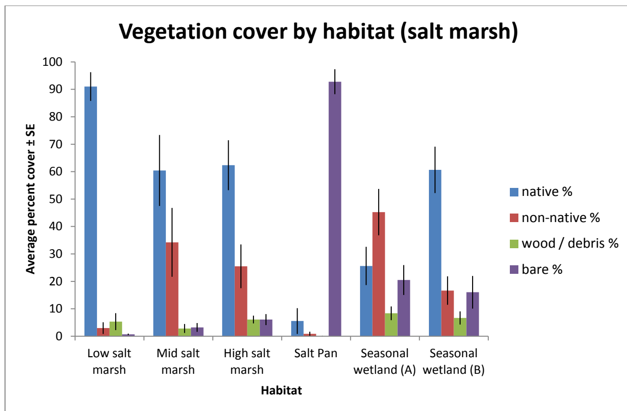
Figure 4.15. Vegetation cover of native versus non-native species averaged for all transect across each salt marsh habitat type.
