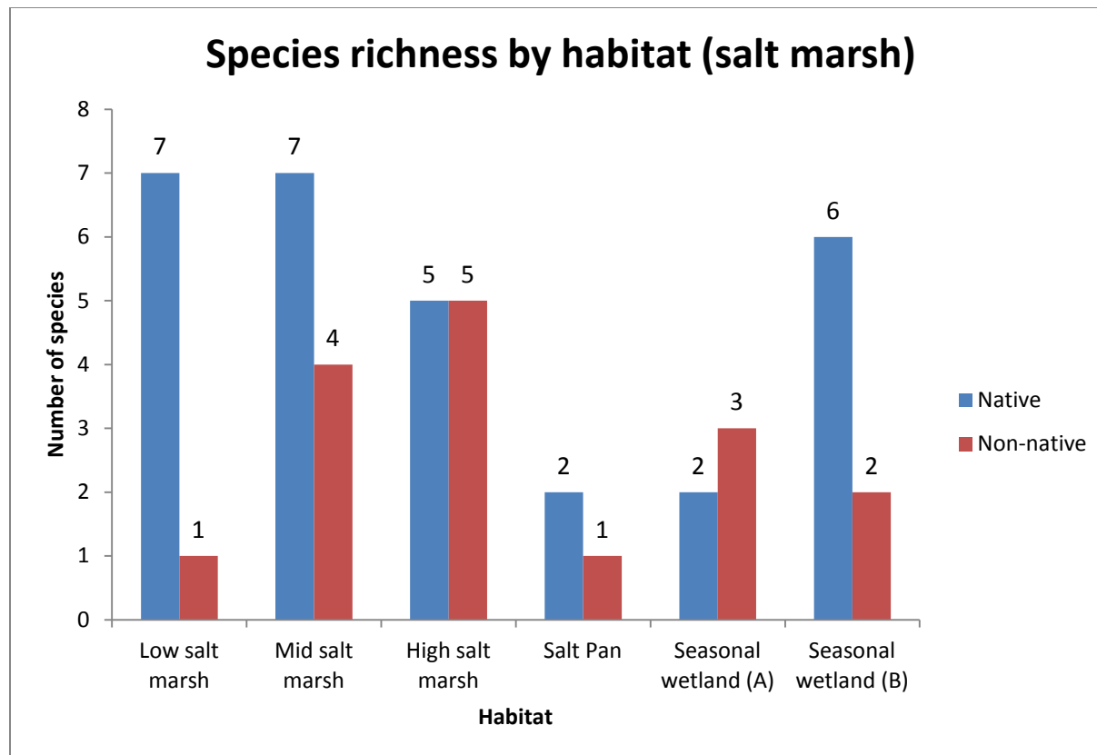
Figure 4.17. Species richness for native and non-native plant species in each of the salt marsh habitats.
