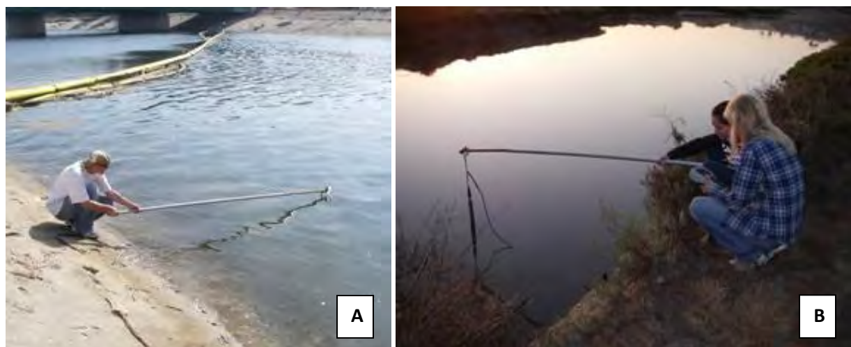
Figure 1.5. Photos depicting: (A) water collection technique, and (B) measurement of in situ water parameter data using YSI 600 QS sonde (photos: SMBRC 2010).
