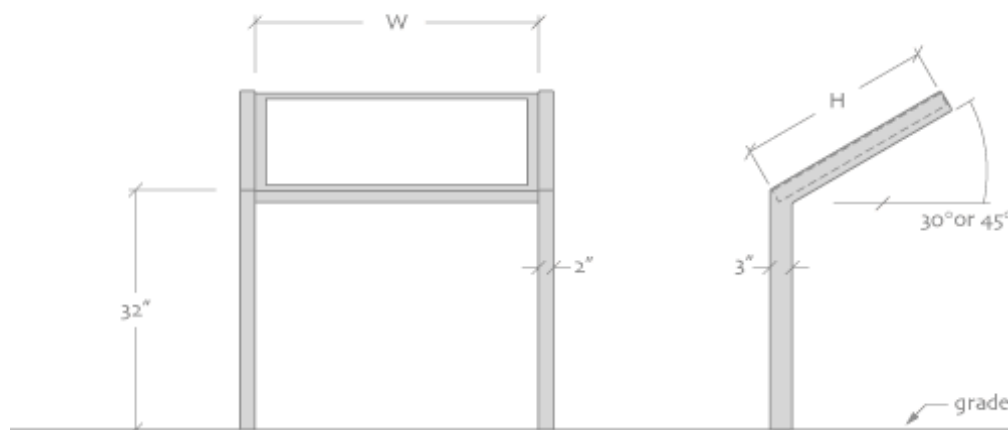
Figure 10. Design of base for interpretive signs.
