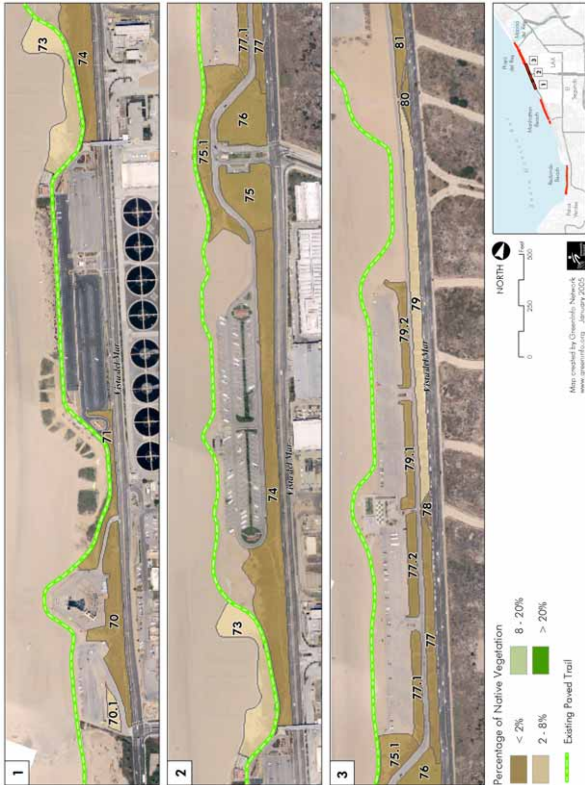
Figure 8. Undeveloped bluffs along Santa Monica Bay showing percent native vegetation (Northern Focus Area, Part 1).
