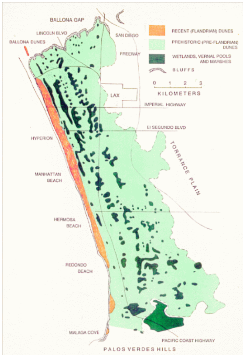
Figure 2. Extent of modern and historic El Segundo dune system (Mattoni 1993a).
