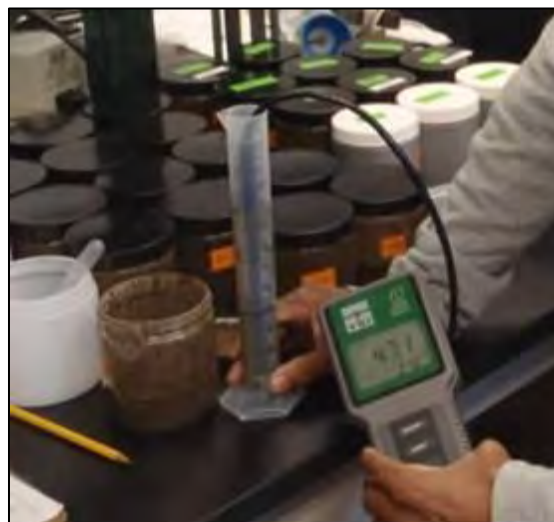
Figure 5. Reading the salinity in a graduated cylinder using a conductivity probe.
